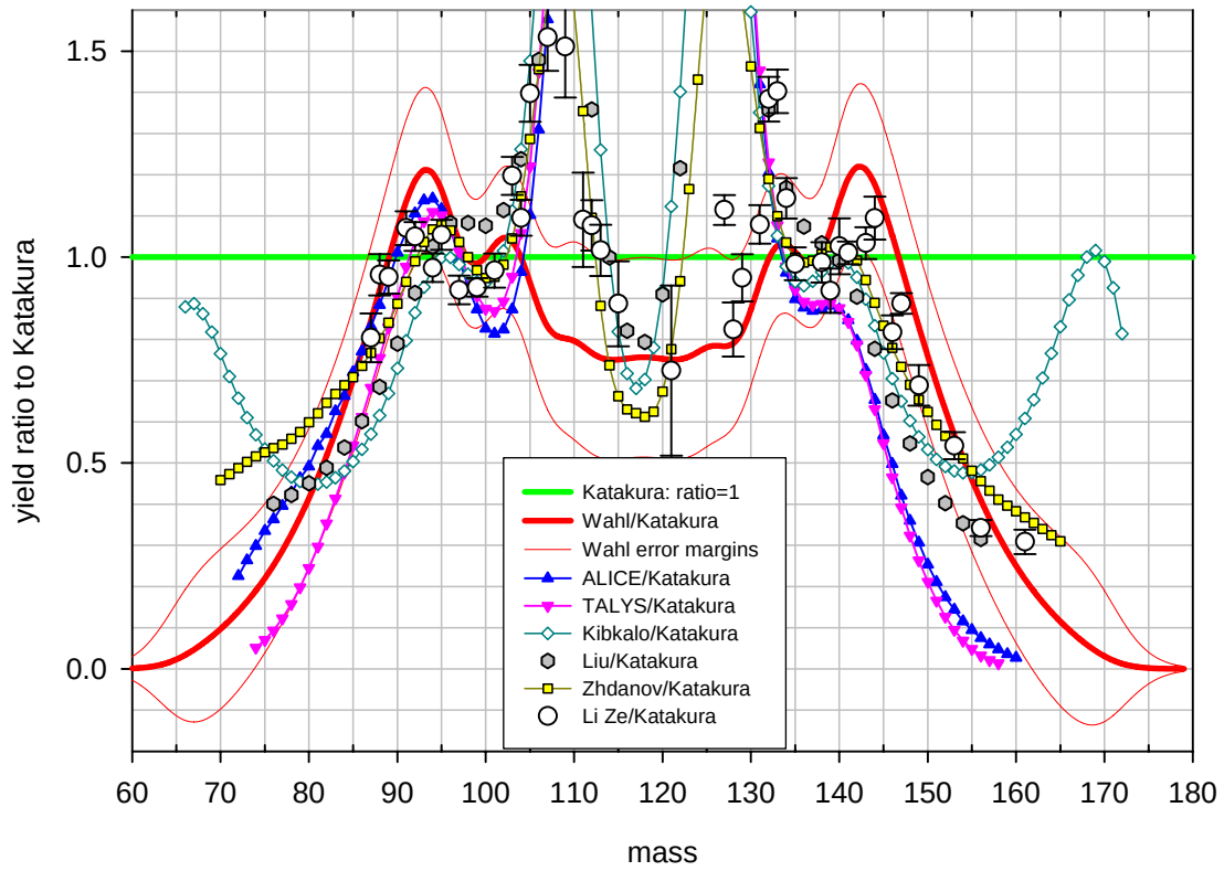
Benchmark A: ^{238}\text{U} at 10.0-11.3 MeV, post neutron emission yield ratios to Katakura's systematics lower graph: high values omitted
